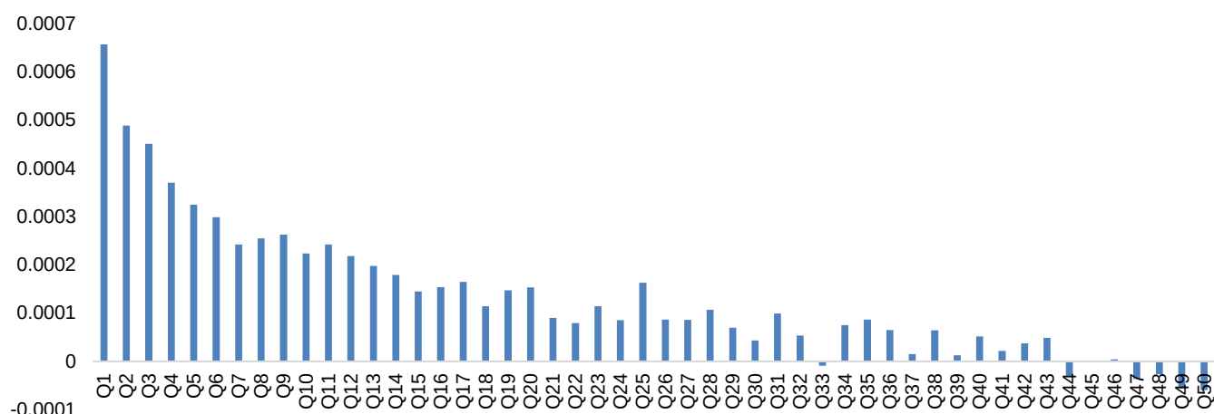
图 3: BuyWithdrew_BuyOrder_ratio_09150920因子在深证A指成分股中的50档分档表现
